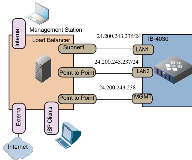
Figure 2 Multiple Interfaces Configured on the Same Subnet on an IB-4030 or IB-4030-10GE Appliance
