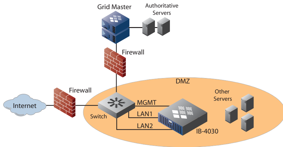
Figure 2-1 IB-4030 or IB-4030-10GE Grid Installation
